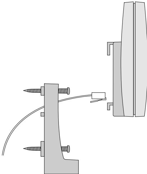
Figure 14 Pull Power Supply Connector and Cable Through Mounting Bracket
